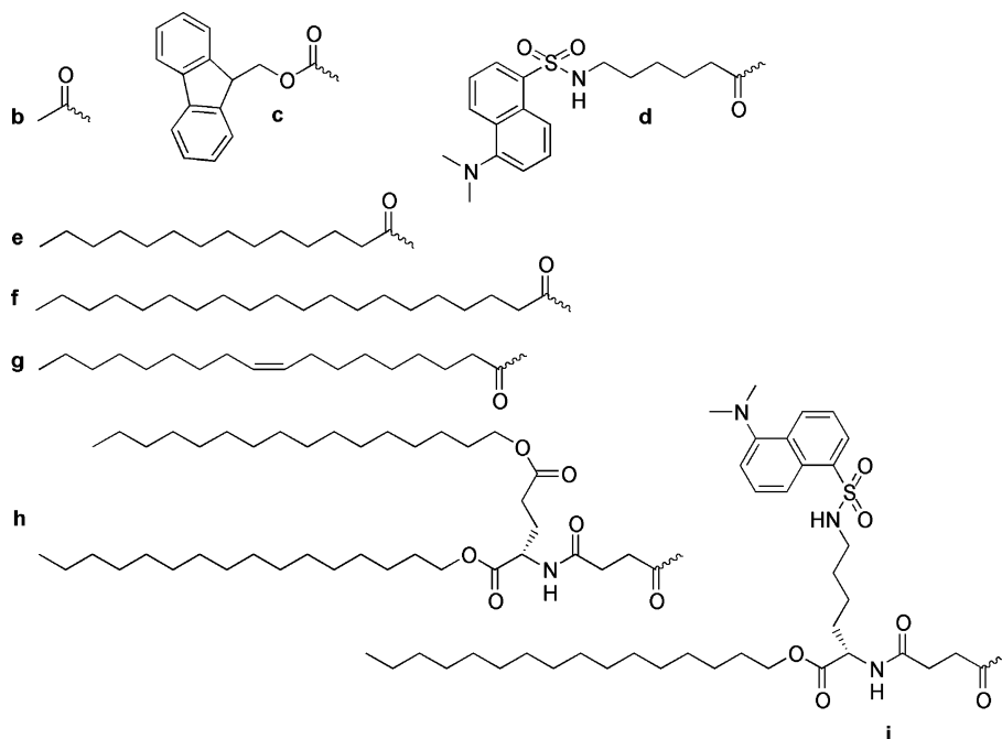
Figure 1. Chemical structures of the N-terminal astressin modifications: (a) none, free N-terminus (H); (b) acetyl (Ac); (c) 9-fluorenylmethyloxycarbonyl (Fmoc); (d) N -dansyl-6-aminohexanoyl (Dans-Ahx); (e) tetradecanoyl (Myr); (f) eicosanoyl (Ara); (g) cis -9-octadecenoyl (oleic); (h) (PalO) 2 Glu inv -Succ-OH; (i) (PalO)Lys inv (Dans)-Succ-OH.
