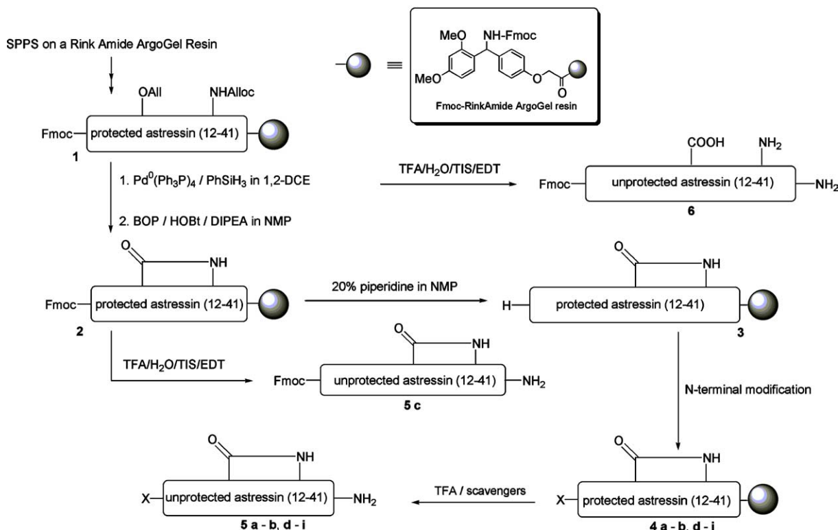
Scheme 1. Schematic overview of the synthesis of the lipo-astressin conjugates.
