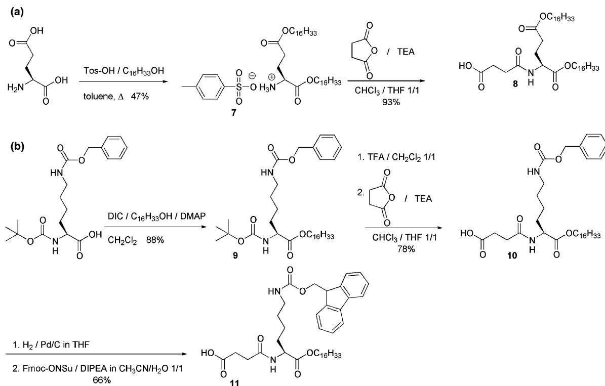
Scheme 2. Schematic overview of the synthesis of the lipidated amino acid residues.
